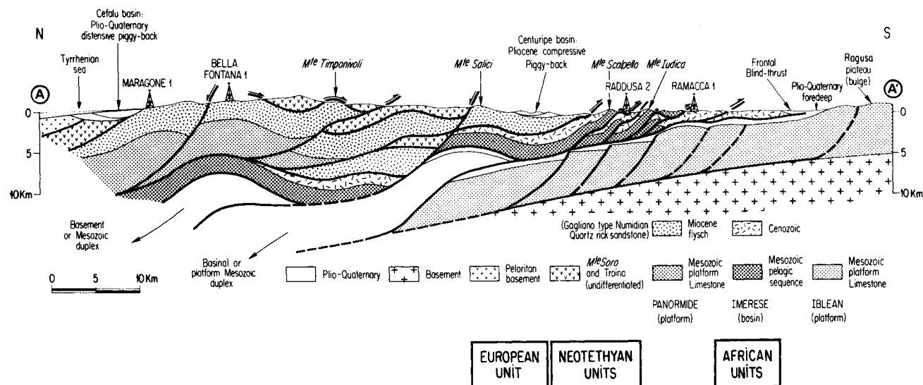
Fig. 5. Generalized cross-section of eastern Sicily (Ragusa to the Tyrrhenian Sea). Well data are taken from Bianchi et al. (1987).
