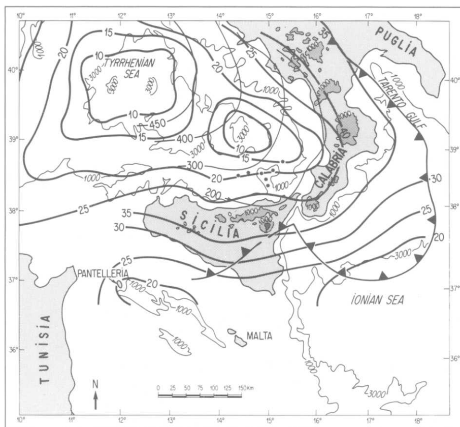
Fig. 1. Crustal thicknesses and physiography of Sicily and neighbouring areas (modified from Gasparini et al. 1982, Rehault et al. 1987). Thickest lines are depths (km) to Moho; smoothly traced thinner lines are depth (km) to top of Benioff zone; irregularly traced thinner lines are bathymetric contours (m).
